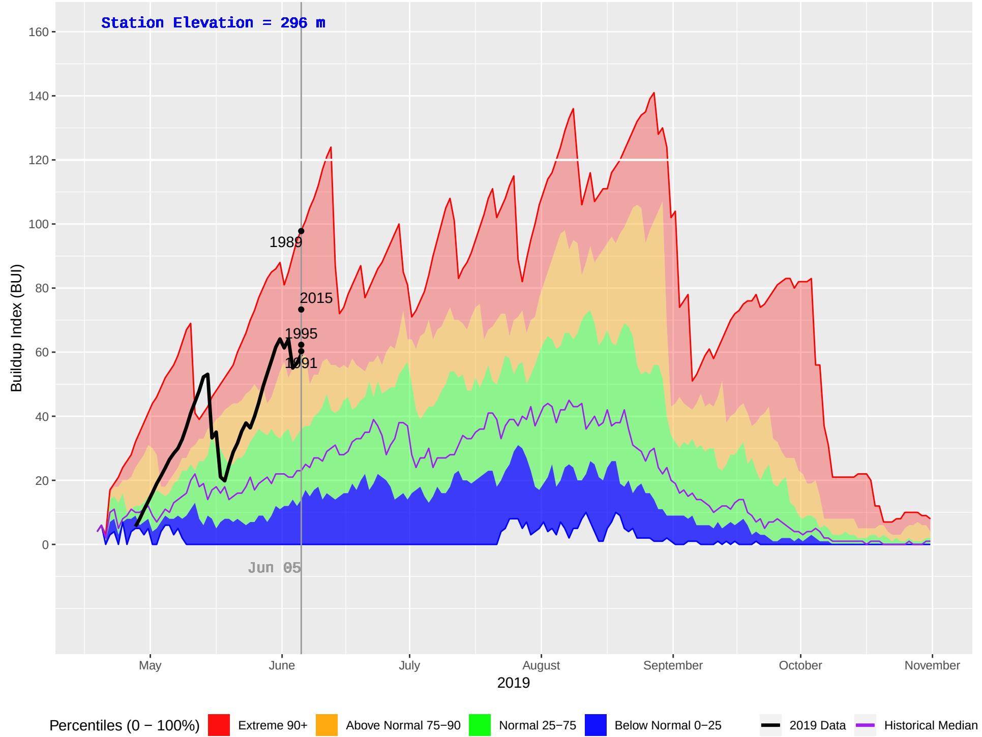
VAN DYKE (430) : Historical (1983–2018), Current (2019) Daily Buildup Index (BUI)
