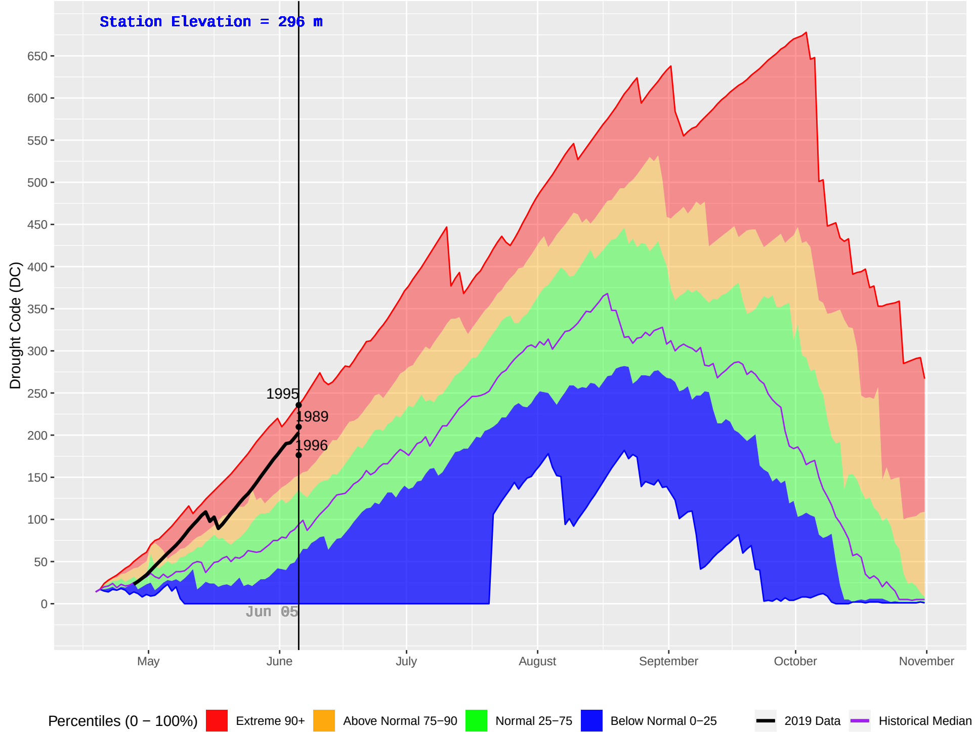
VAN DYKE (430) : Historical (1983–2018) and Current (2019) Daily Drought Code (DC)
