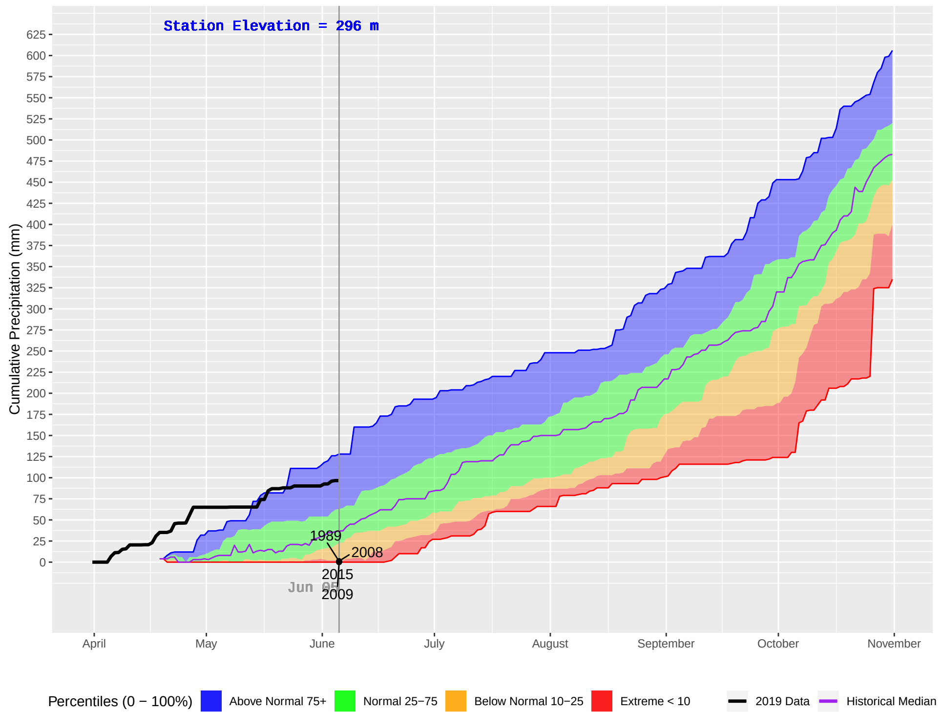
VAN DYKE (430) : Historical (1983–2018), Current (2019) Daily Cumulative Precipitation
