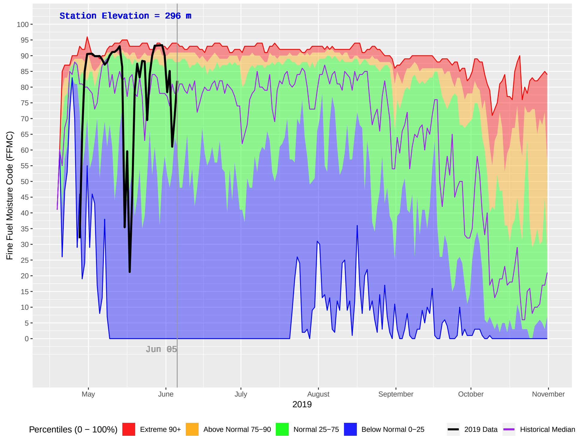
VAN DYKE (430) : Historical (1983–2018) and Current (2019) Daily Fine Fuel Moisture Code (FFMC)
