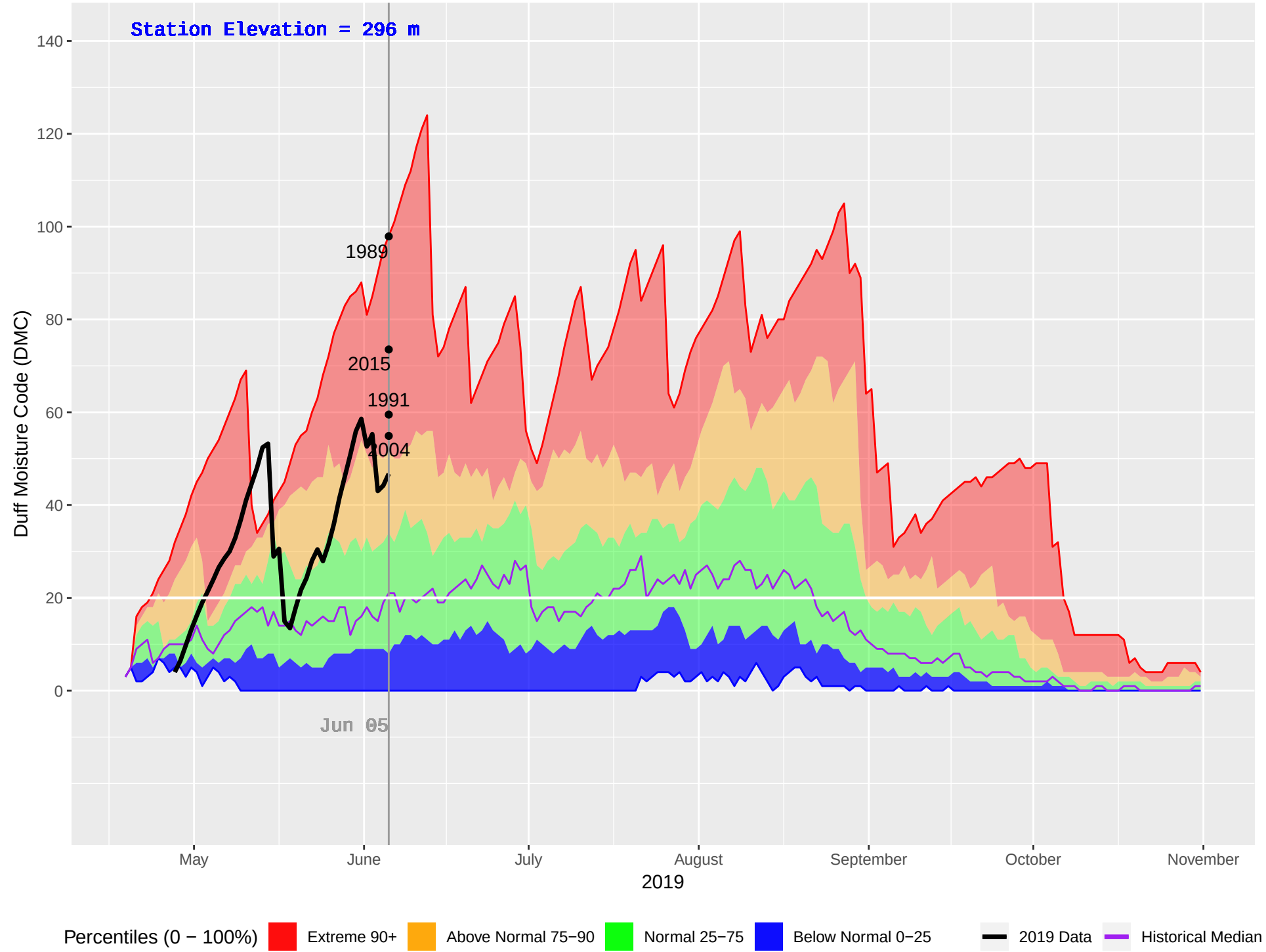
VAN DYKE (430) : Historical (1983–2018), Current (2019) Daily Duff Moisture Code (DMC)
