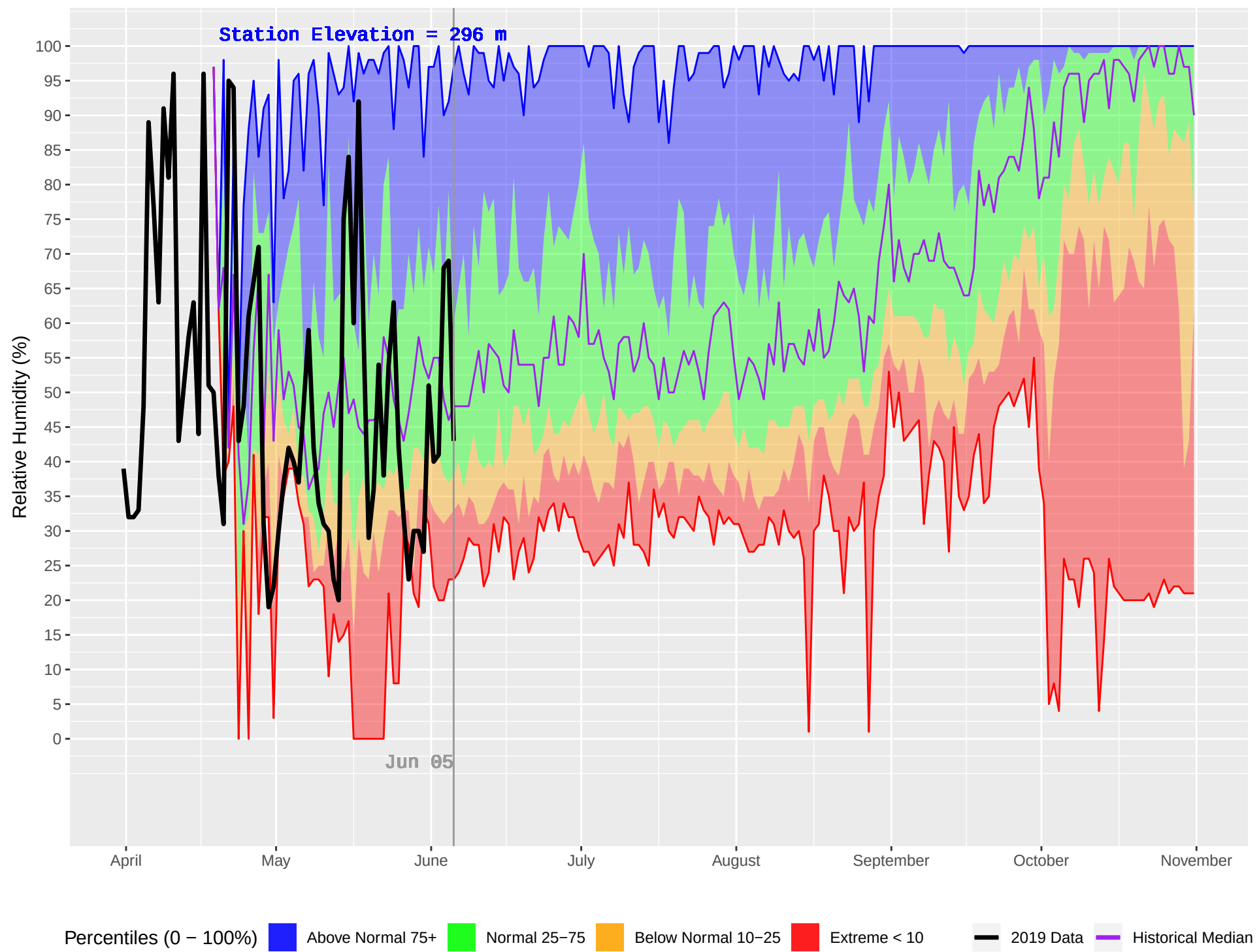
VAN DYKE (430) : Historical (1983–2018) and Current (2019) Daily Relative Humidity
